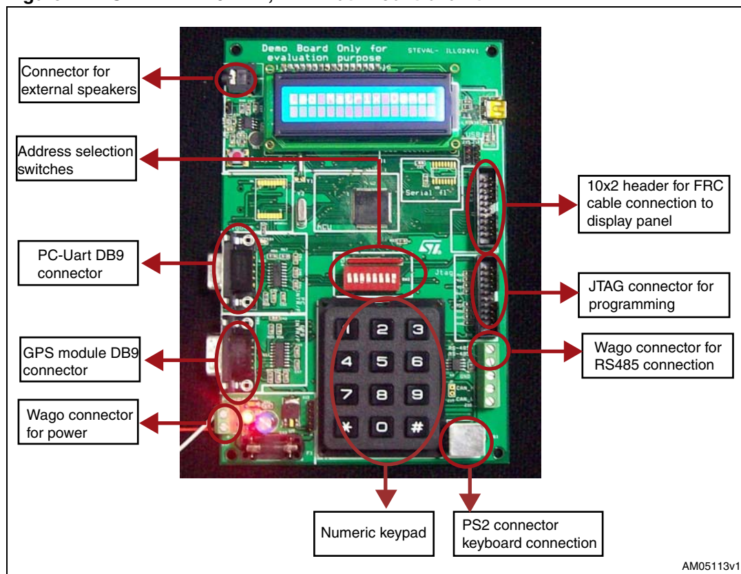
Figure 2. STEVAL-ILL024V1, LED matrix control unit
