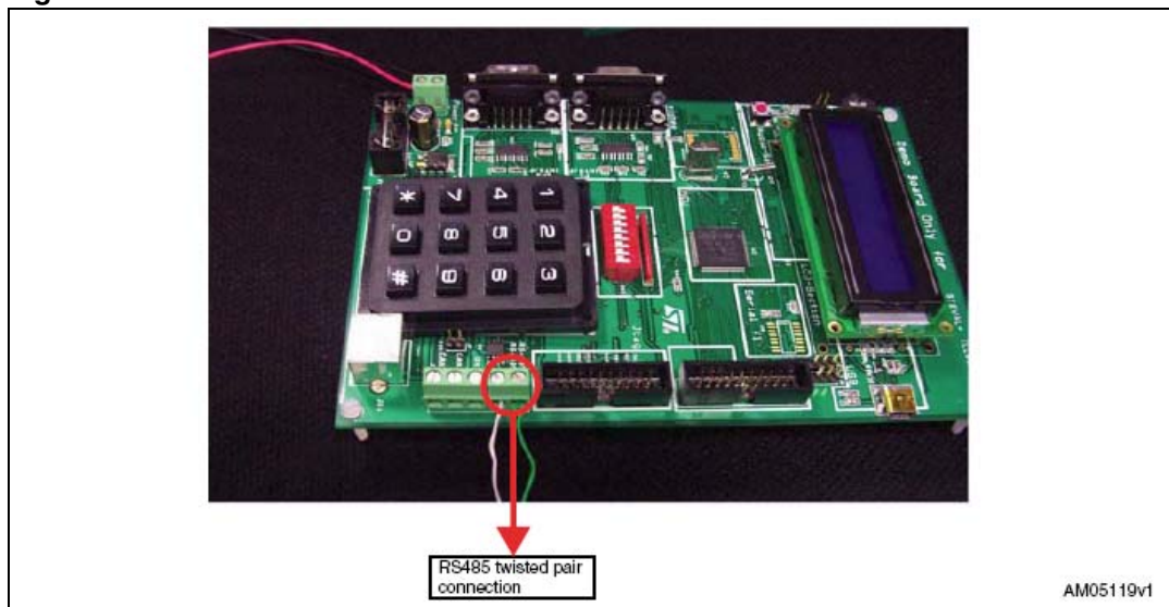
Figure 7. RS485 communication
